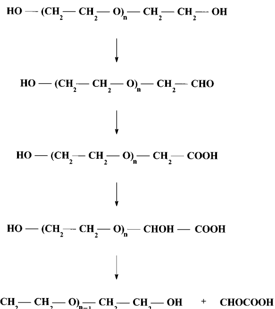
FIG. 9. Oxidative mechanism for ether scission of PEG by a synergistic mixed culture, as proposed by Kawai (53).
