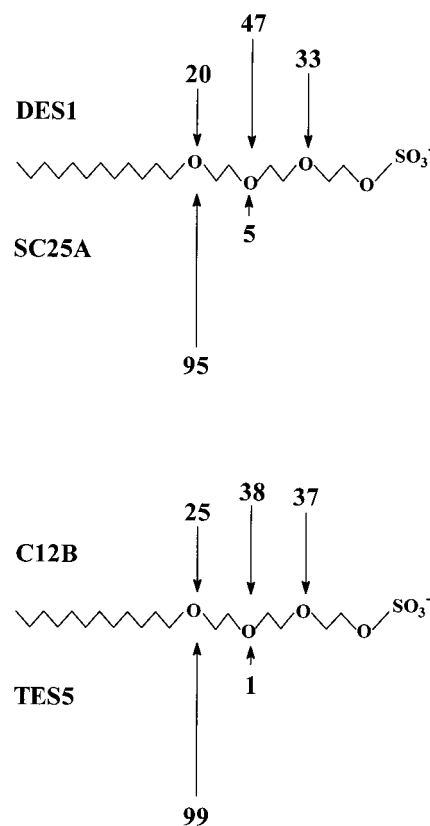
FIG. 2. Regioselectivity of the ether-cleaving activities in four bacteria which biodegrade alkyl ethoxylate and alkyloxy sulfate surfactants. Arrows indicate the point of cleavage, and their lengths indicate the relative percentages of the substrate ether bond cleaved at that position (values quoted at base of arrow).
